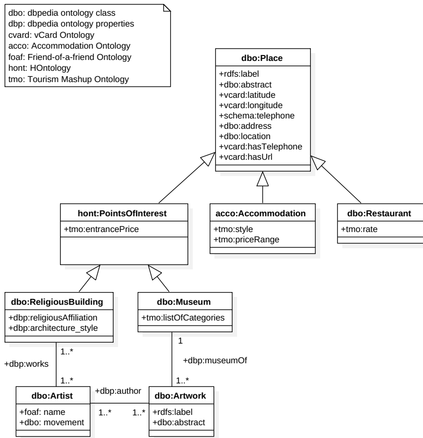
Figure 5: The tourism mashup view fragment representing places.
