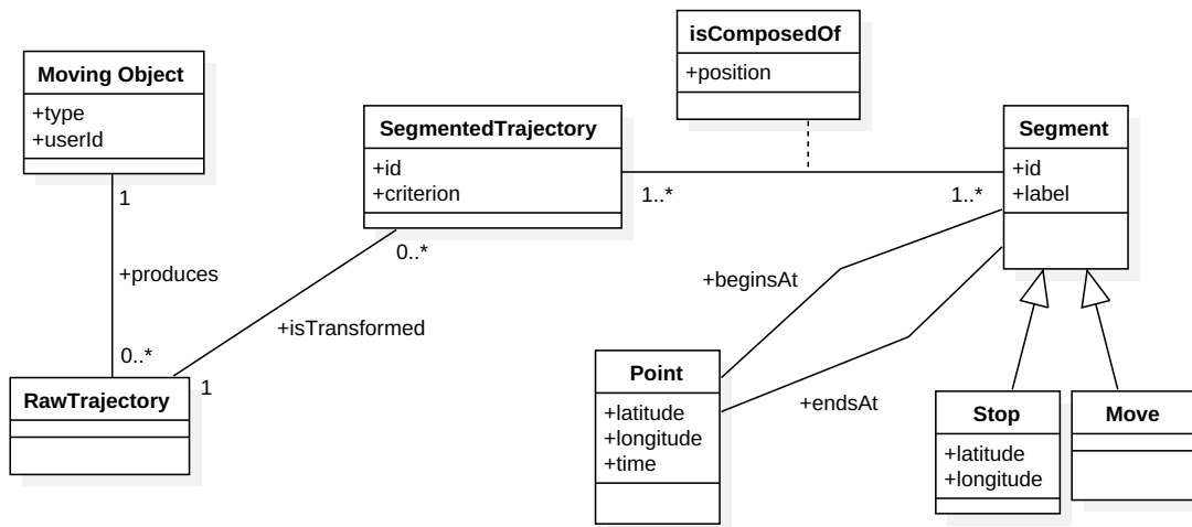
Figure 3: The Segmented Trajectory Ontology
