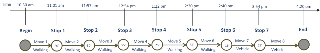
Figure 4: The running example segmented trajectory
