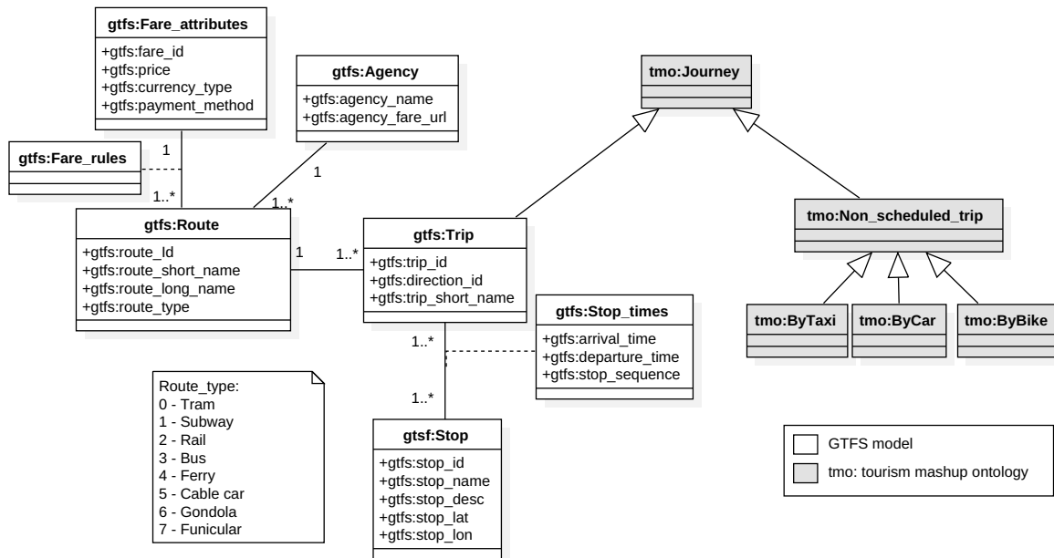
Figure 6: The Tourism Mashup view fragment about transportation
