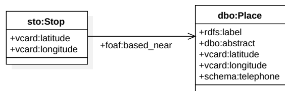
Figure 7: The Stop Enrichment
