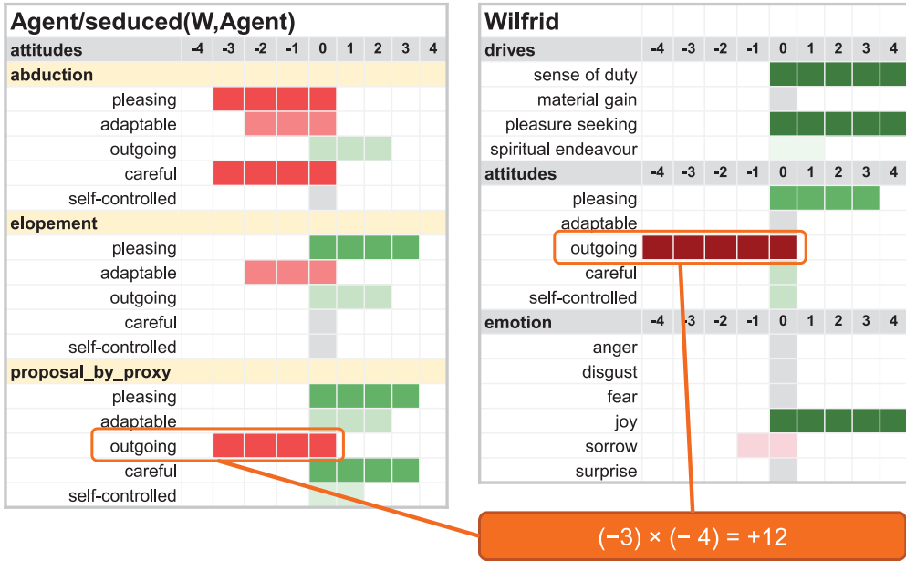
Fig. 1. Obtaining a ranking value for the plan, considering the plan’s values and the character’s attitude weights.
