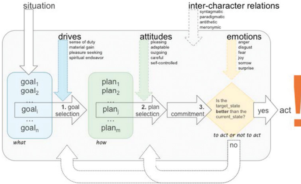
Fig. 2. Our three-step decision-making process.
