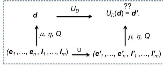
Fig. 4. Incremental view maintenance problem
