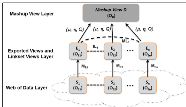
Fig. 1. Three Level Ontology-Based Framework.
