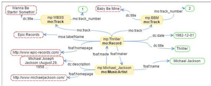
Fig. 6. New state of the mashup view
