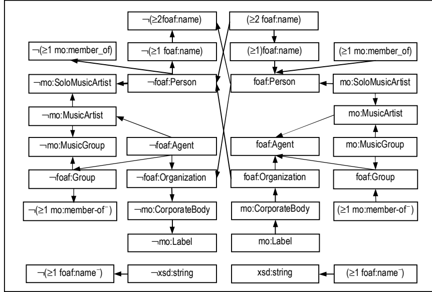
Fig. 2. The graph G(\Sigma_{APO}) representing the constraints of APO .
