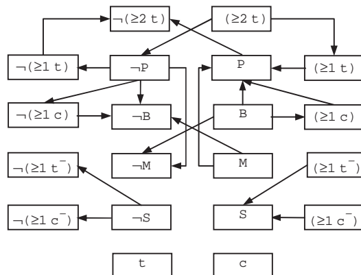
Fig. 6. The graph G(\Sigma) that represents \Sigma .
