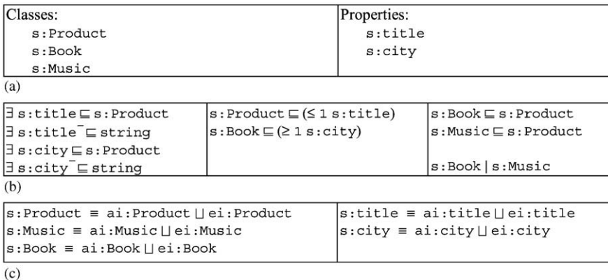
Fig. 4. (a). Vocabulary of the Sales mediated schema. (b). Constraints of the Sales mediated schema. (c). Mediated mapping.
