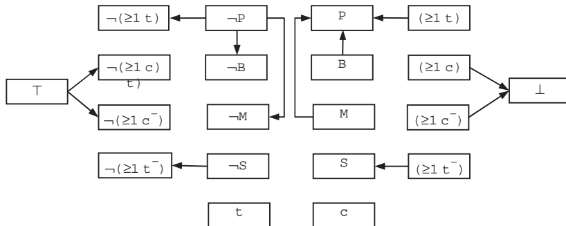
Fig. 7. The graph G(\Phi) that represents \Phi .
