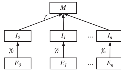
Fig. 1. Components of a mediation environment.
