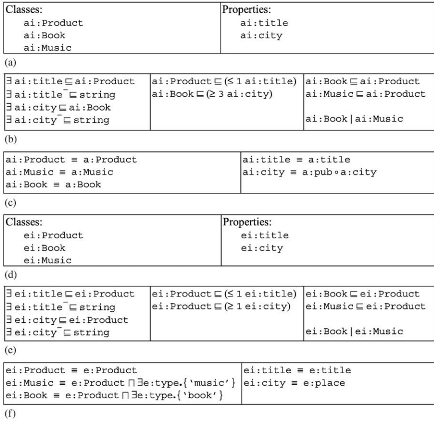
Fig. 3. (a). Vocabulary of the Amazon import schema. (b). Constraints of the Amazon import schema. (c). Local mapping from the Amazon export schema to Amazon import schema. (d). Vocabulary of the eBay import schema. (e). Constraints of the eBay import schema. (f). Local mapping from the eBay export schema to the eBay import schema.
