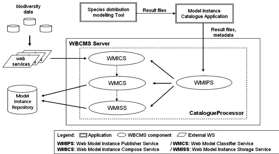
Figure 4 Catalogue Processor Context
