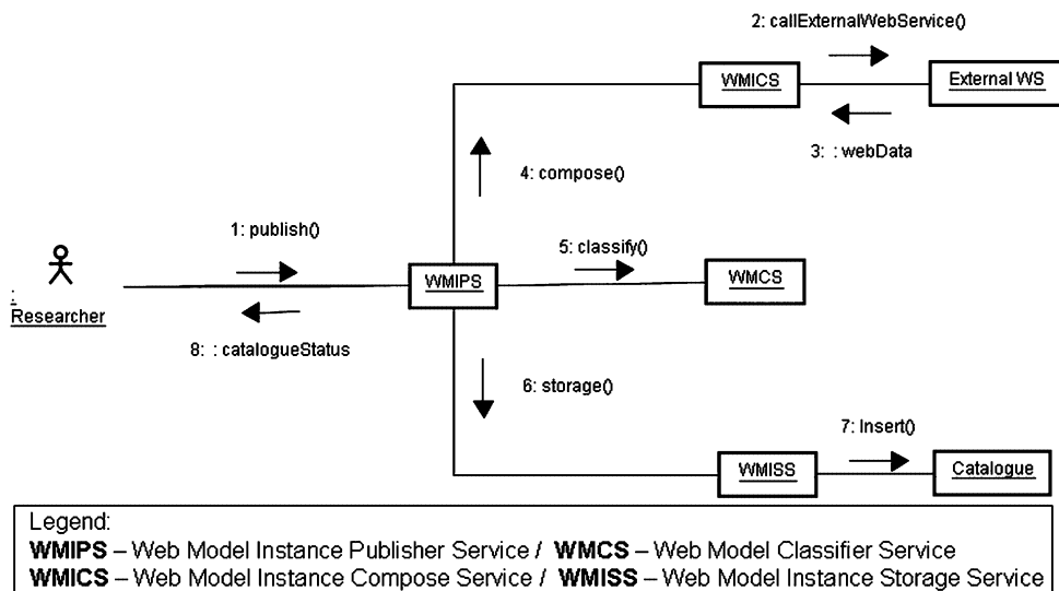
Figure 5 Catalogue Processor collaboration diagram
