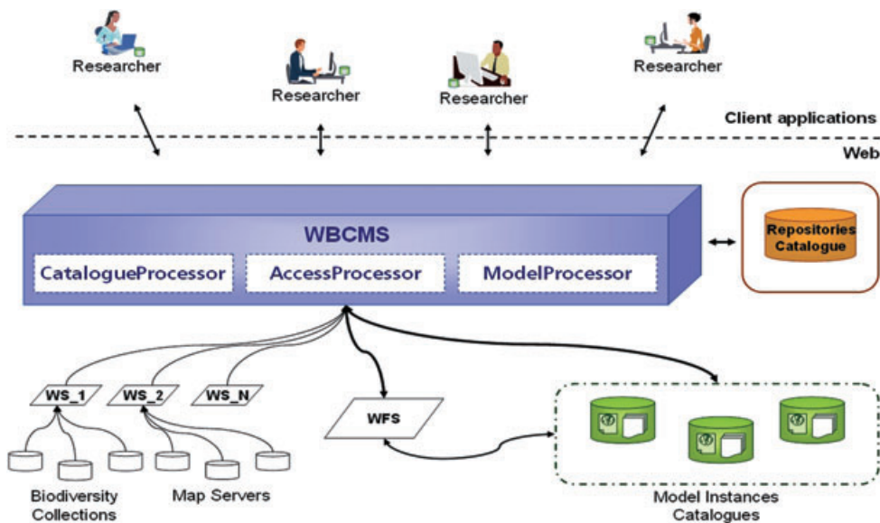
Figure 3 WBCMS Architecture
