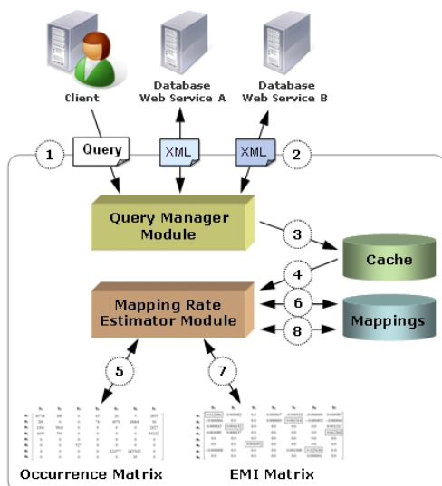
Figure 1: The matching process.
